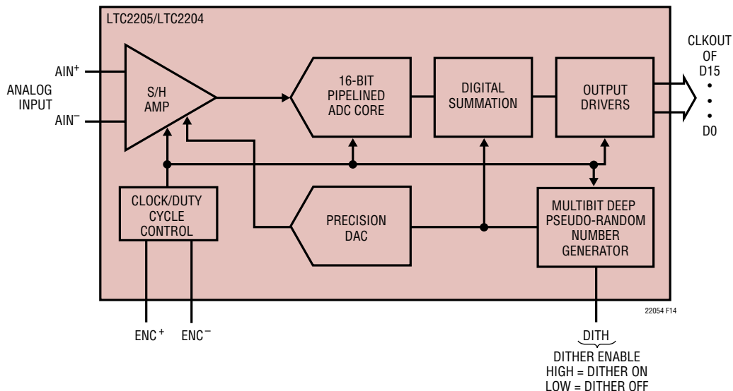
Figure 14. Functional Equivalent Block Diagram of Internal Dither Circuit
